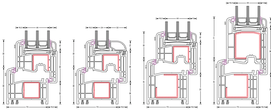
8001 - 8095 8001 - 8095 rounded glazing bead 8012 - 8095 8012 - 8081
